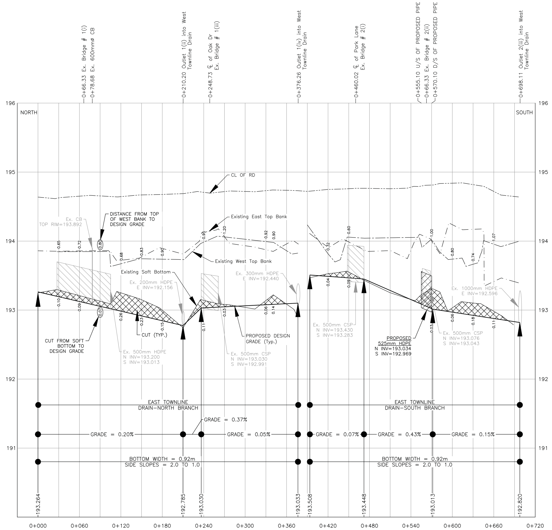
EAST TOWNLINE DRAIN-NORTH & SOUTH BRANCH-PROFILE
