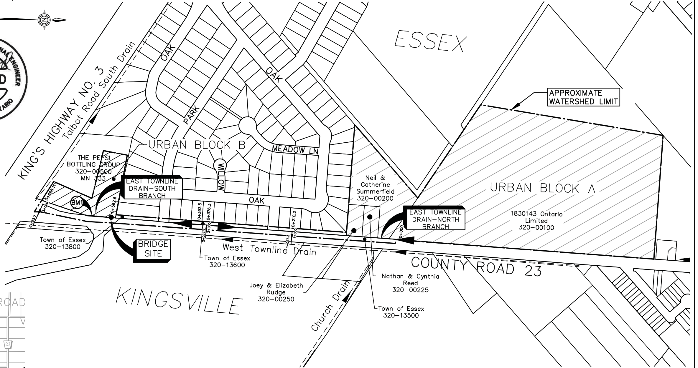
WATERSHED PLAN Scale = 1:2,000
