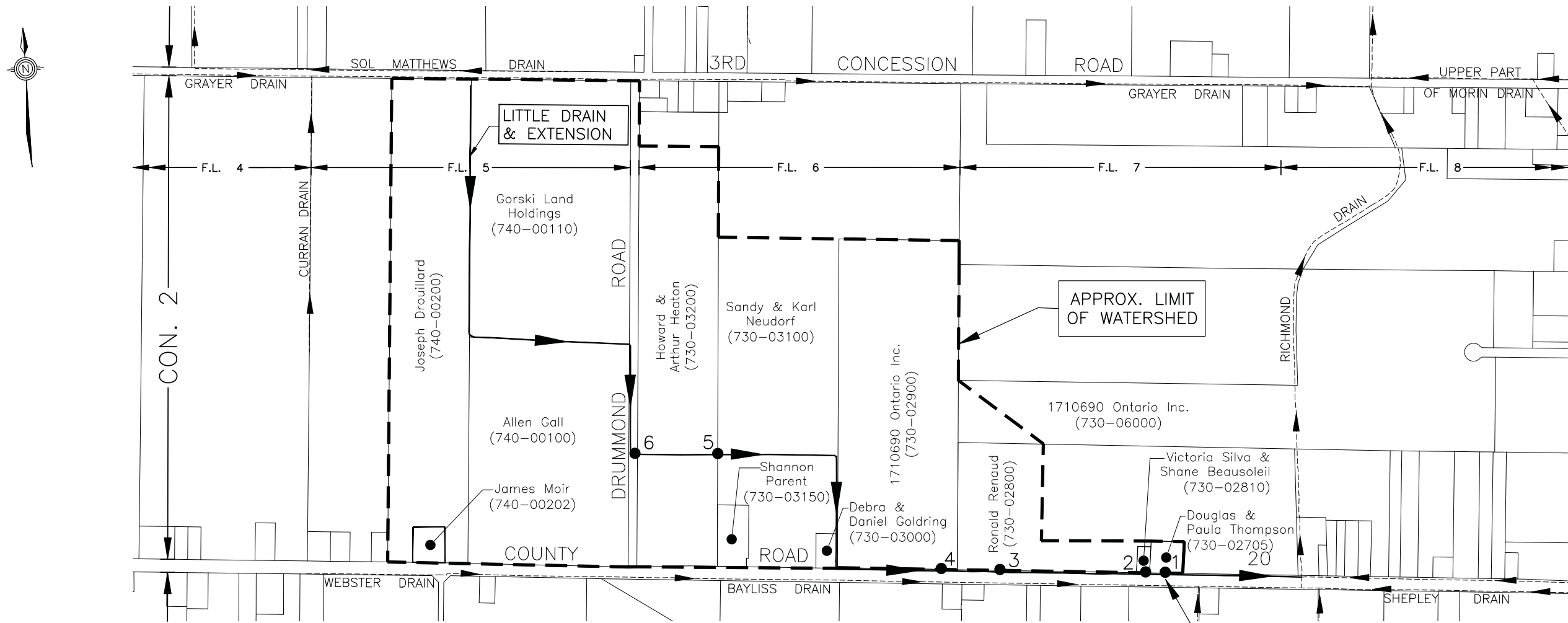
WATERSHED PLAN SCALE = 1:5000
