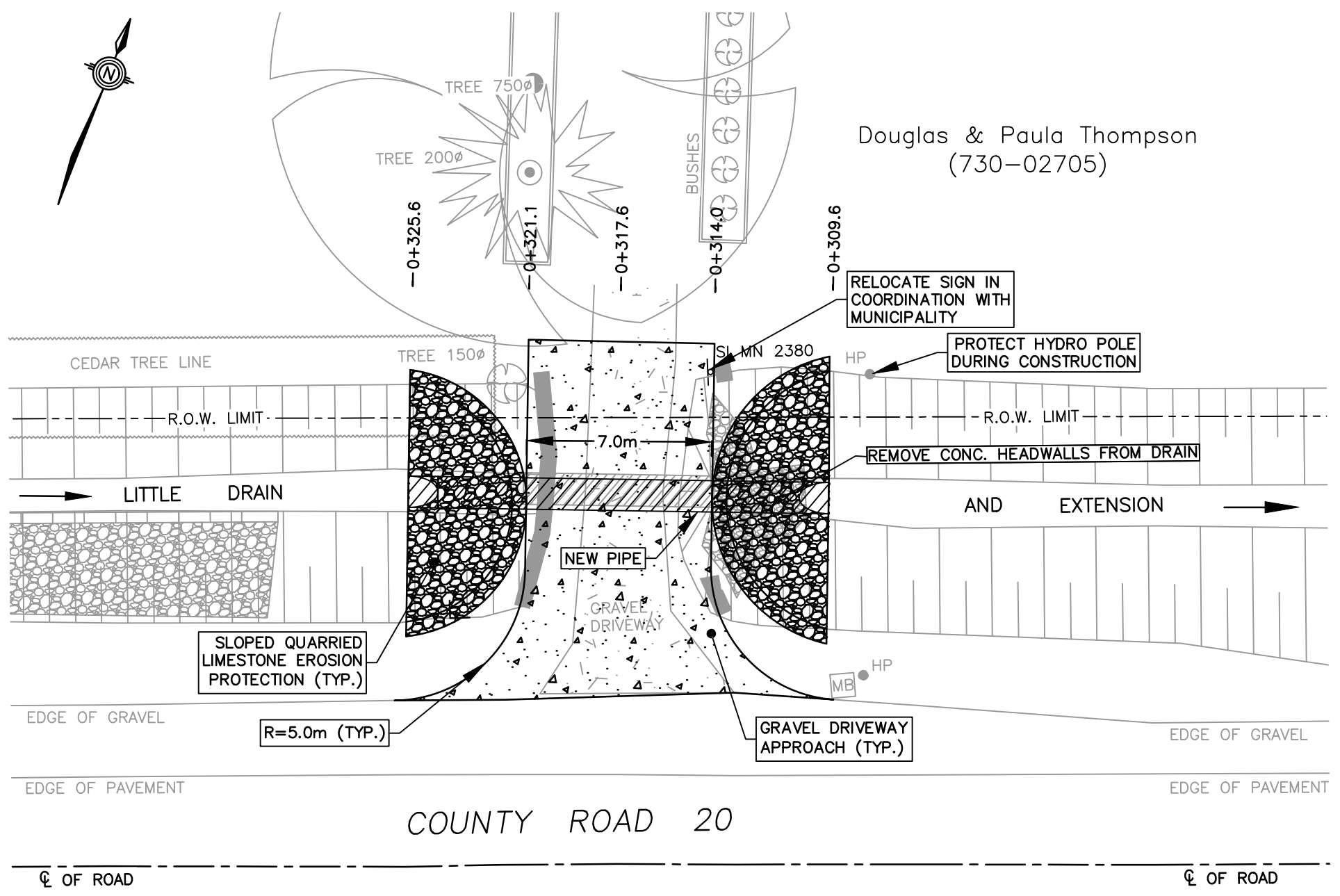
BRIDGE PLAN SCALE = 1:200
