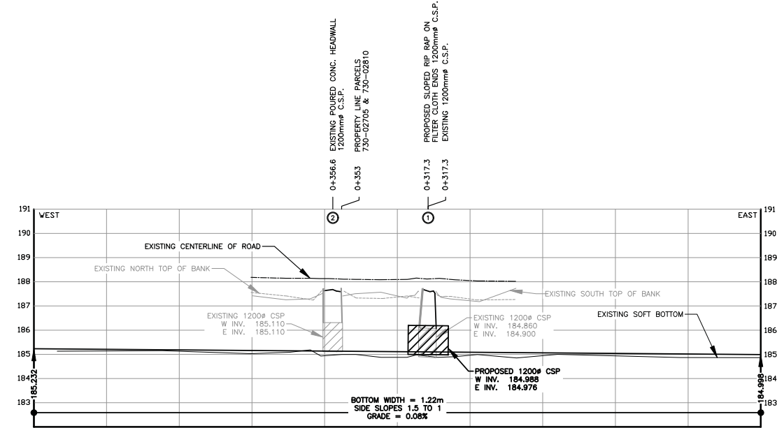
PROFILE - LITTLE DRAIN SCALE=1:1000 hor. 1:100 vert.
