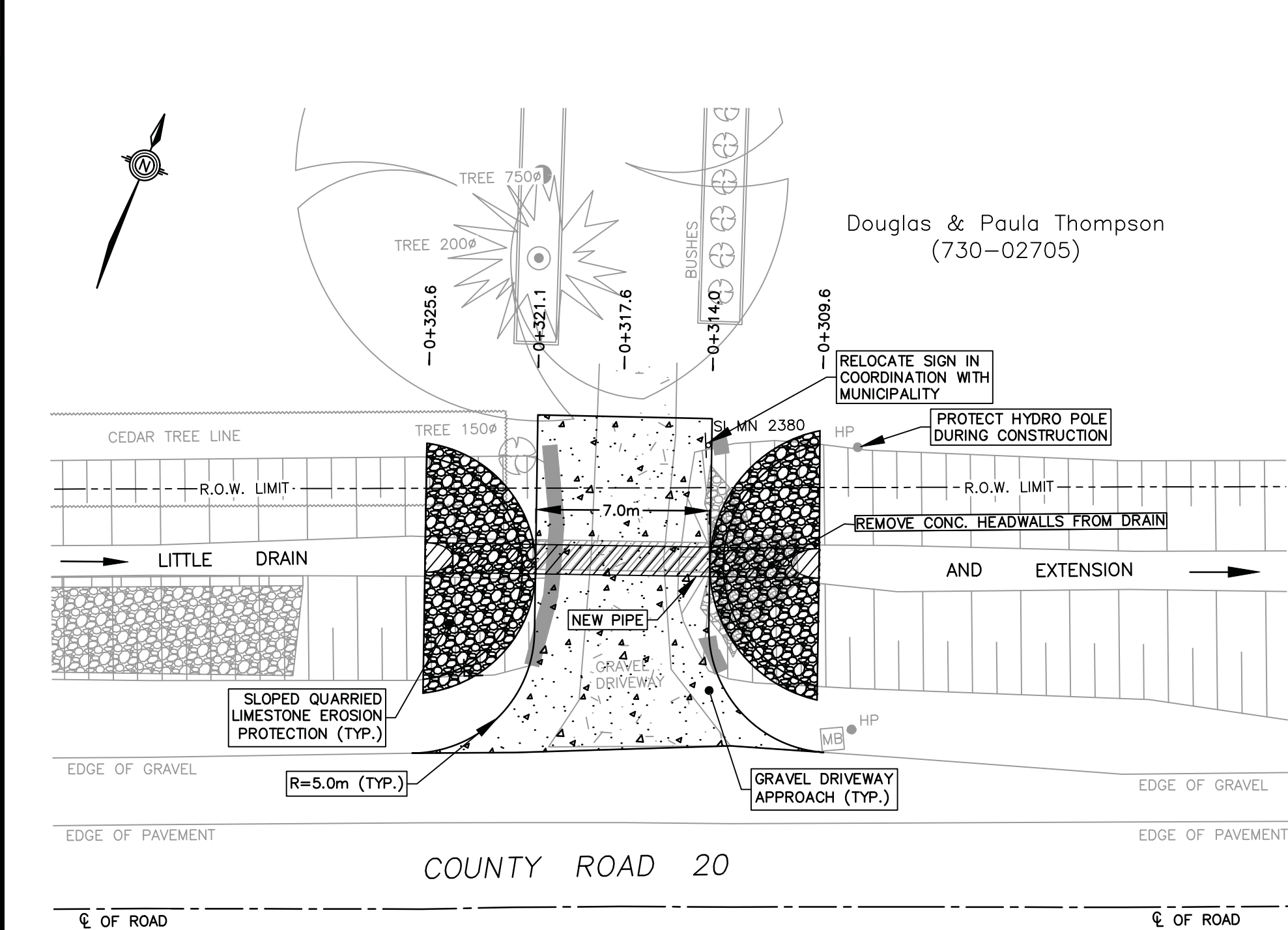
BRIDGE PLAN SCALE = 1:200
