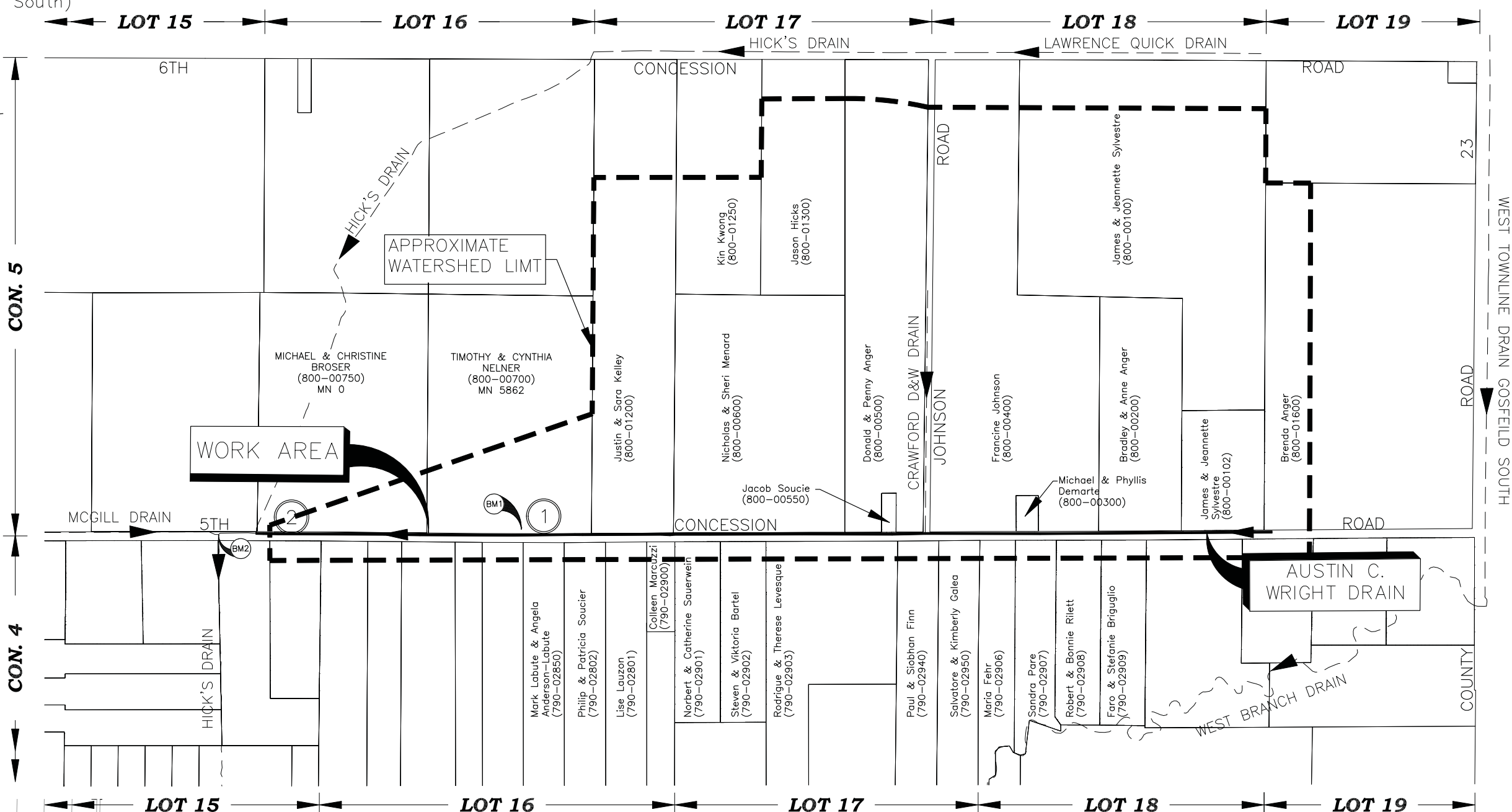
WATERSHED PLAN SCALE = 1:5,000
