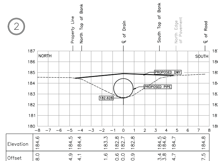
℄ OF PROPOSED CULVERT – STA. 0+131.56 SCALE = 1:100
