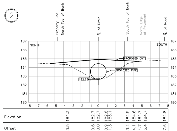
EAST END OF DRIVEWAY – STA. 0+135.81 SCALE = 1:100
